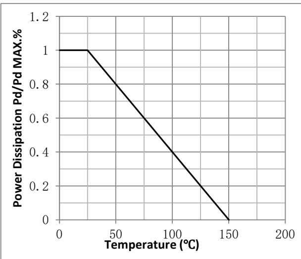
Fig.3 Power Dissipation
